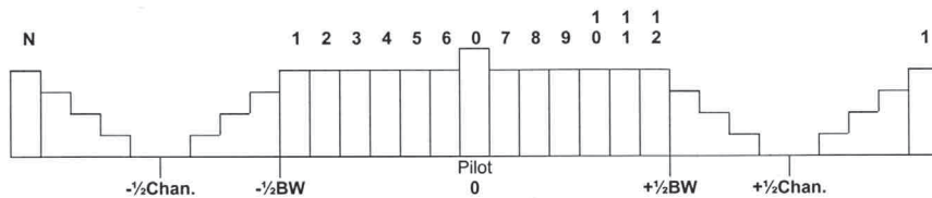
Fig 1—13-carrier transmission channel format (not to scale).
